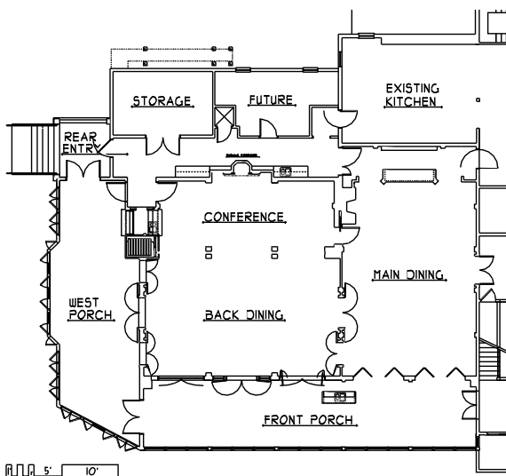
ALTERNATE FLOOR PLAN (OPEN)
